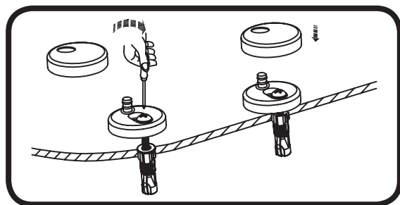
2. Rotate the brackets until you are happy with the toilet seat alignment on the pan.
